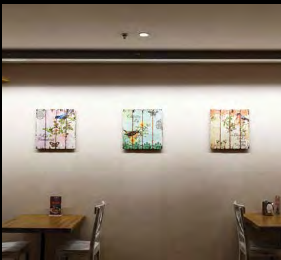
Single asymmetric LED lines provided excellent even light distribution on the wall whereas wide beam angle tracklights chosen to illuminate the beverage shelves.
